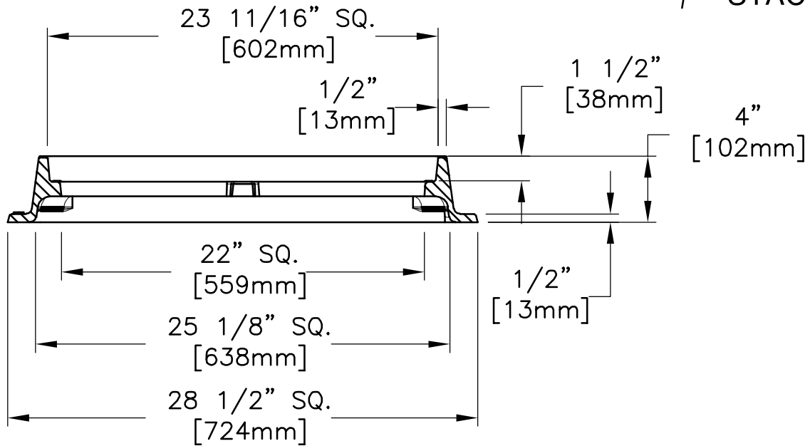
SECTION VIEW
