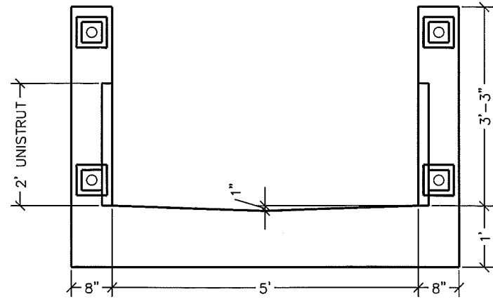
END VIEW 10' UTILIDOR SECTION
