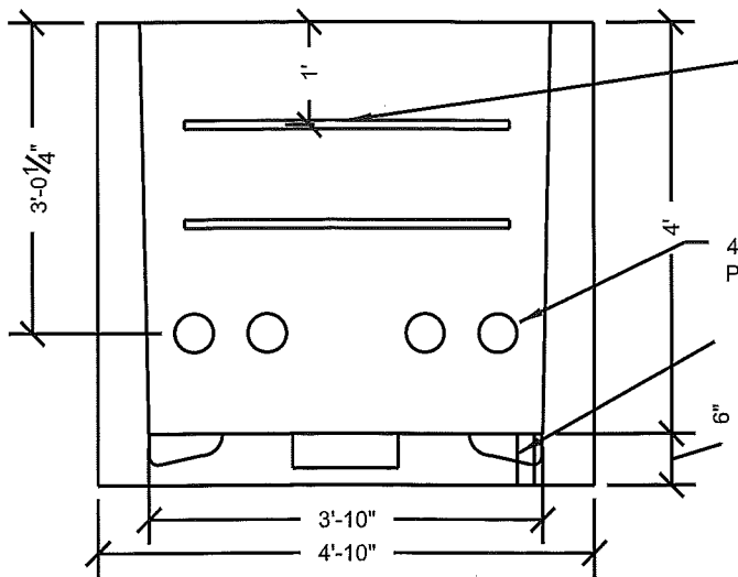
VAULT - SIDE VIEW WITHOUT LID
